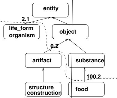
Figure 3: ATCM for 'eat' object slot.
